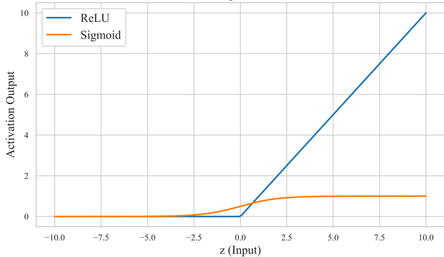
ReLU vs. Sigmoid Activation
